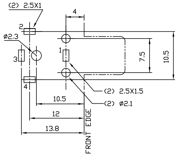
PCB LAYOUT
