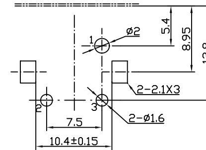
DIMENSIONS OF PC BOARD HOLES(COMMEND) BOTTOM VIEW
